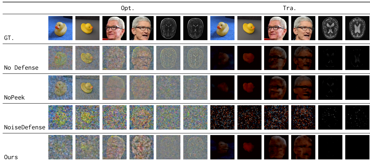
Figure 11: Comparison of reconstructed images from the optimization-based attack (Opt.) and training-based attack (Tra.) under different defense mechanisms.
