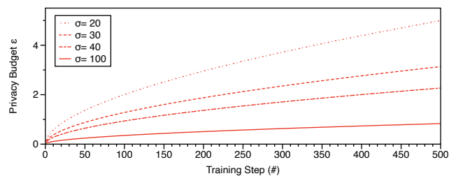
Figure 13: Estimate of \epsilon during DP-SGD fine-tuning for different noise multipliers \sigma , with \delta = 10^{-5} .
