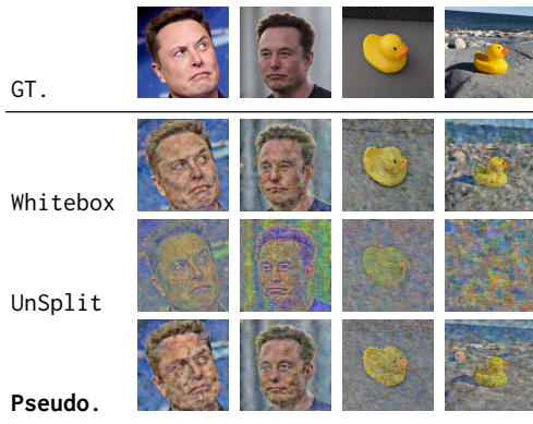
Figure 5: A comparison of reconstructed images with different levels of the adversary’s knowledge of the client’s model.
